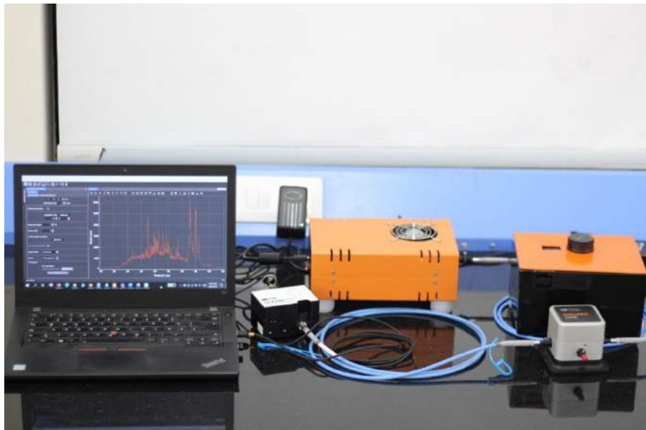
FLUORESCENCE SPECTROMETER
